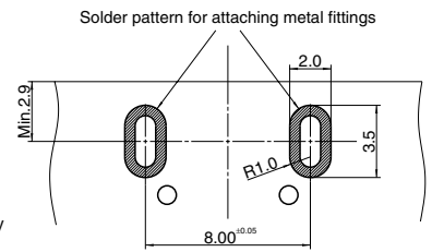
Recommended PC board pattern (BOTTOM VIEW)
