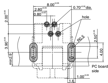
Recommended PC board pattern (BOTTOM VIEW)
