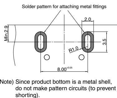
Recommended PC board pattern (BOTTOM VIEW)
